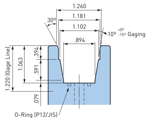
S=4.331" (110mm)
