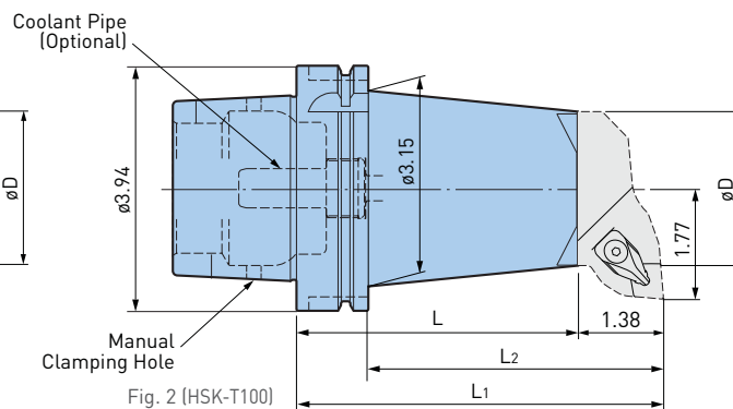
Fig. 2 (HSK-T100)
