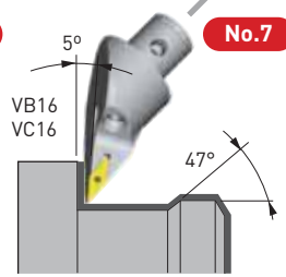
S50-SVLBR-33075-16 -SVLBL-33075-16
